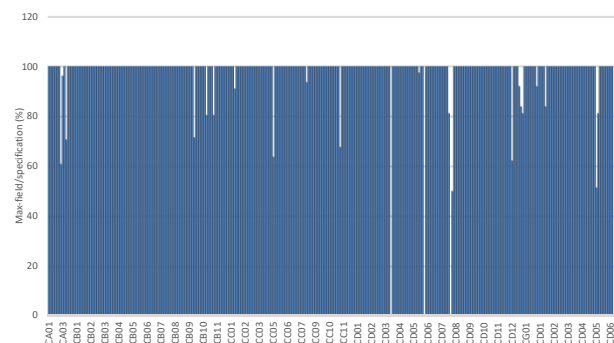
Figure 9: Maximum E_{acc} for each cavity as of May 2023.
